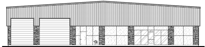
SOUTH ELEVATION
